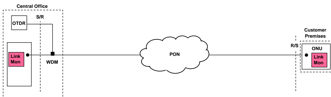
Figure 7 – Application of link-monitoring functions for PON optical-layer management.
