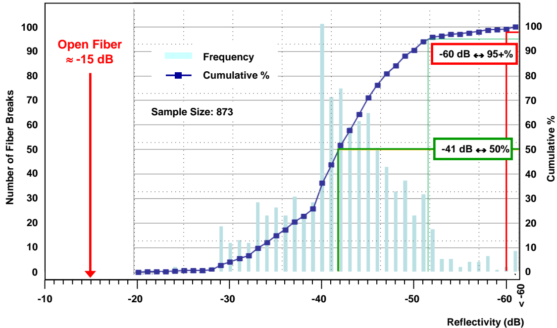
Figure 15 – Statistical distribution of fiber-break optical-return-loss values (adapted from [12], used with permission).
