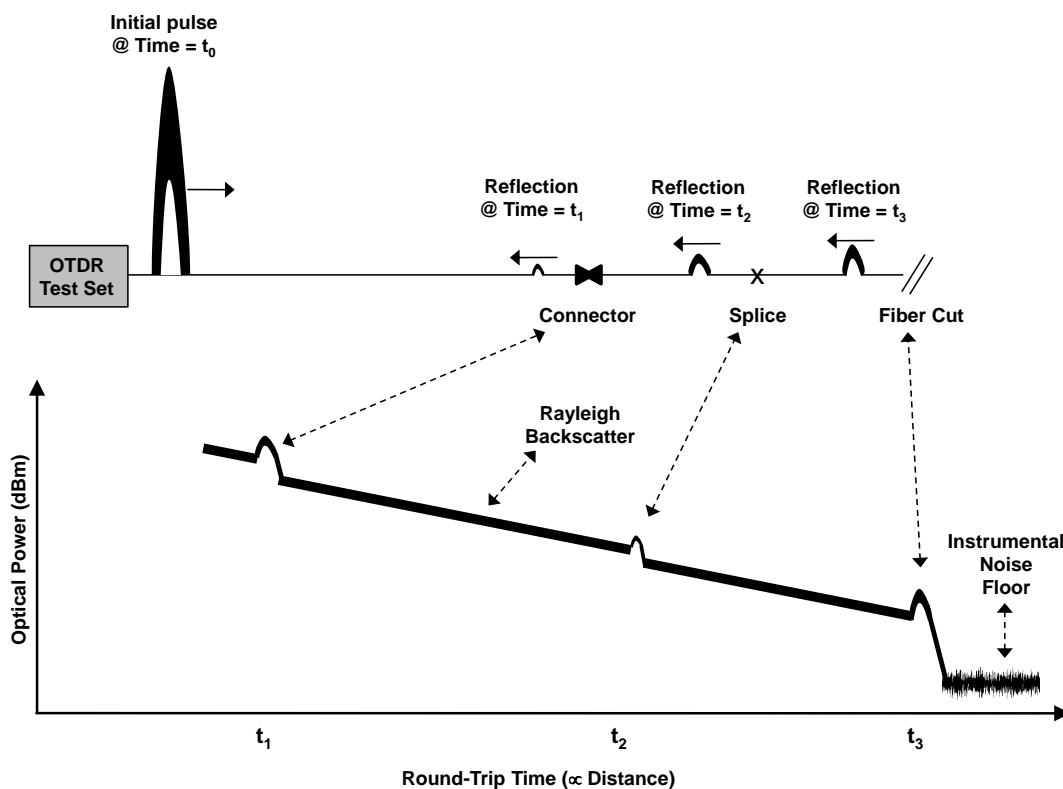
Figure 11 – OTDR characterization of a point-to-point link.
