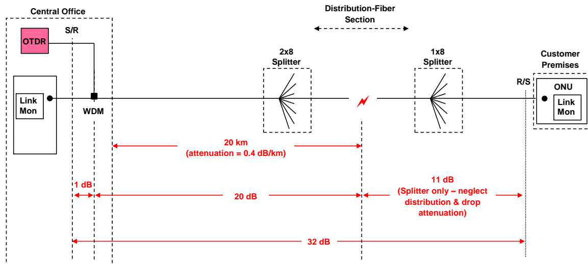
Figure 9 – Use of OTDR to locate a distribution-fiber impairment.
