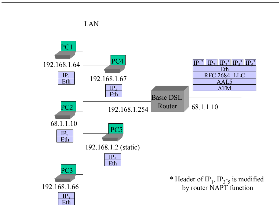
Figure 6 / TR-124 - Example of Router in 2684 Bridged Mode with DHCP Server On
