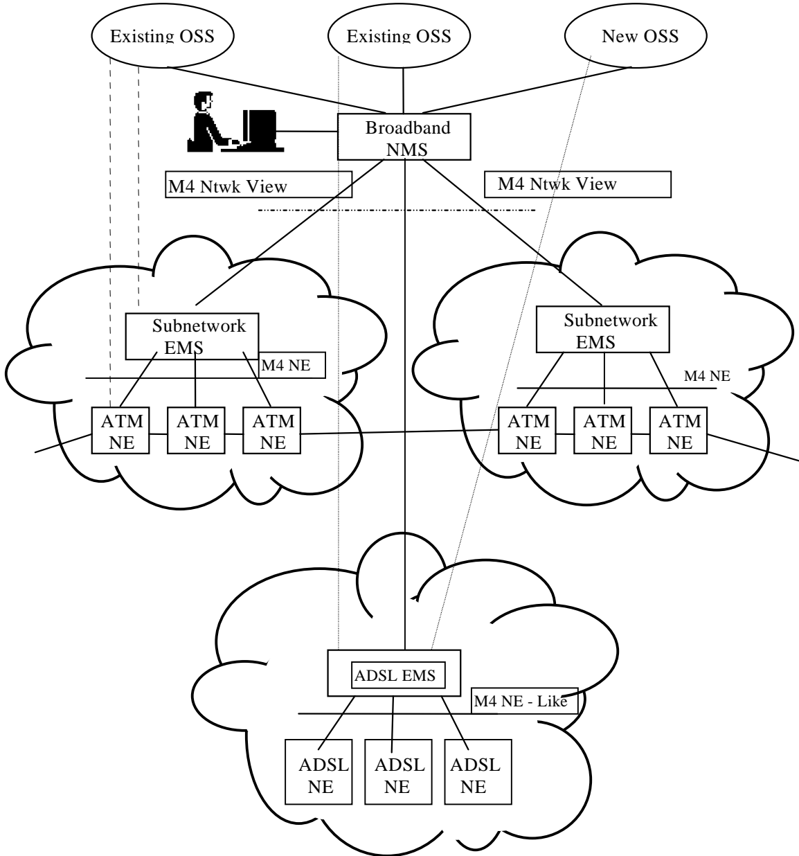
Figure 1. Example of Broadband NMS Environment
