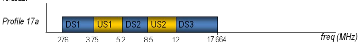
Figure 5 - Example band plans for profile 17a
