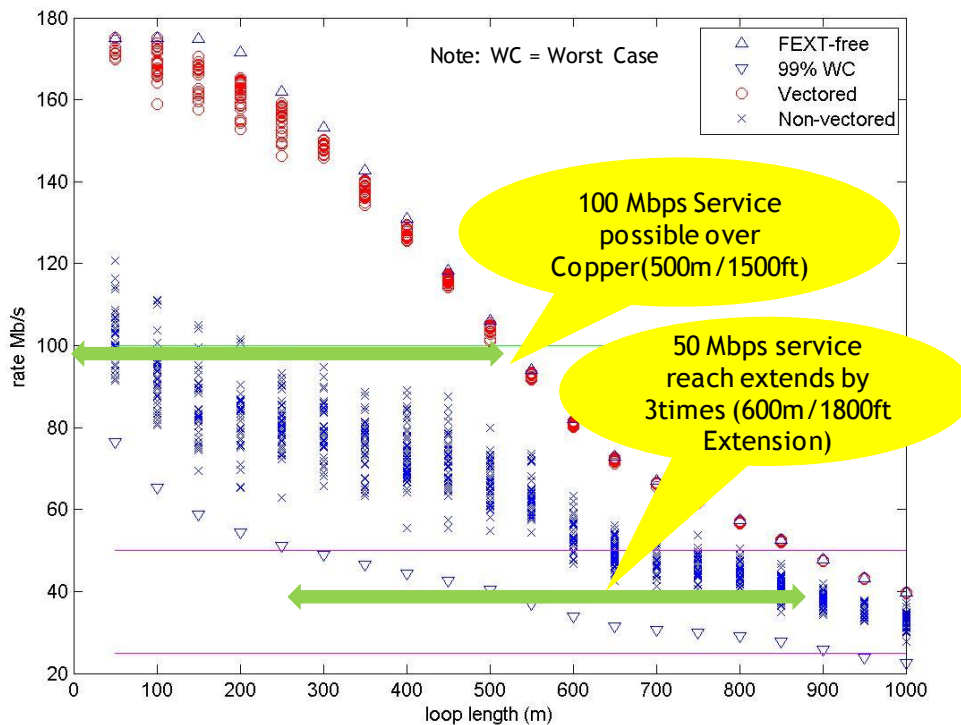
Figure 6 - Downstream Rates – Profile 17a, 26 AWG, -136 dBm/Hz noise, 80 users, and 47 cancelled
