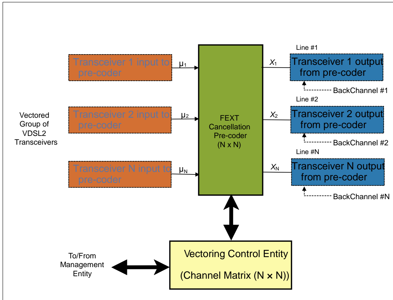
Figure 4 - Downstream FEXT Cancellation Pre-coding in DSLAM
